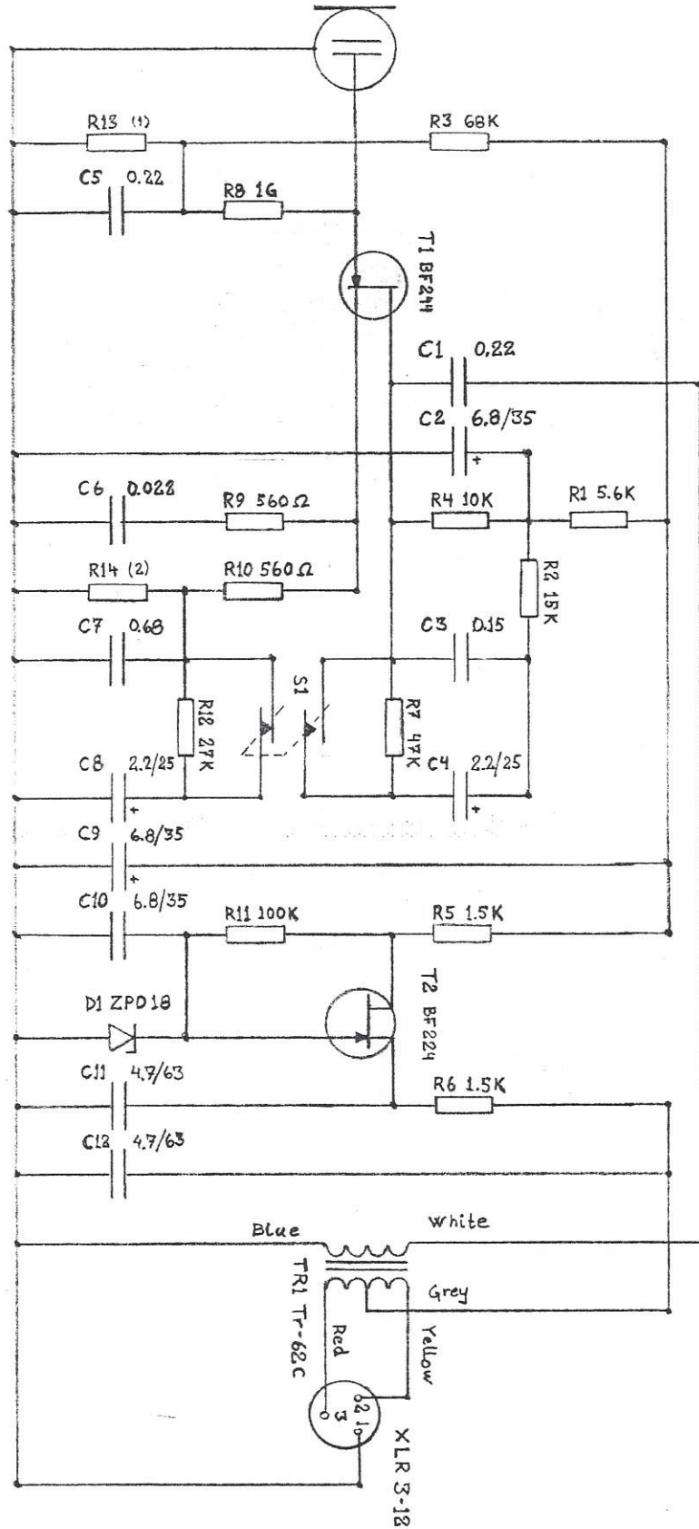
circuit diagram
