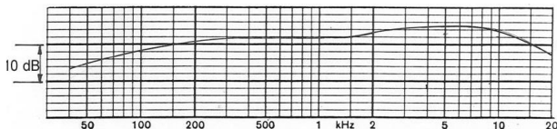
Cardioid
