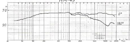
Typical frequency response curve of HM-49
