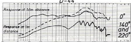
Typical frequency response curve of D-44
